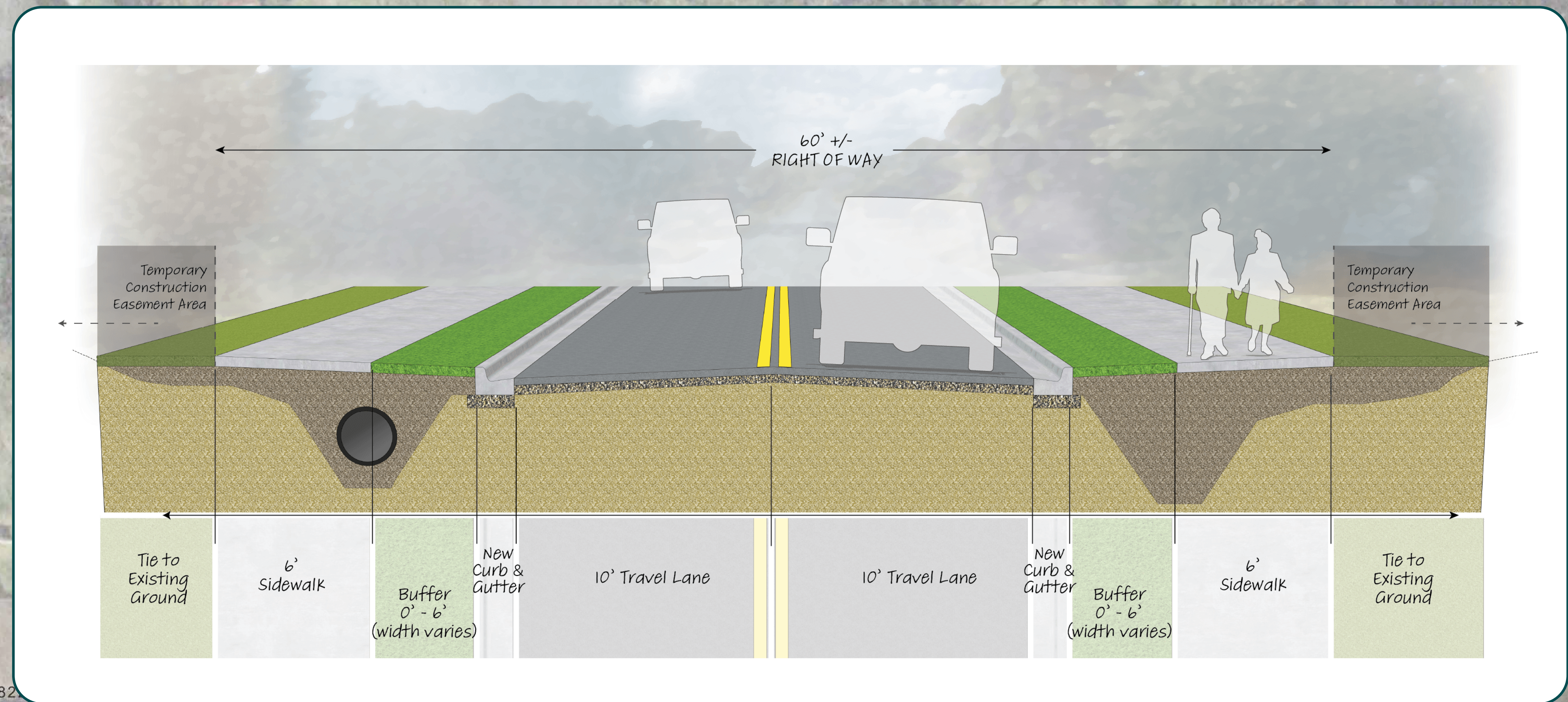
TYPICAL SECTION
